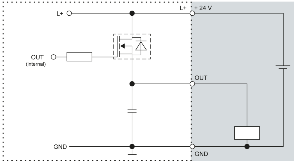
Fig. 15: Principle circuit diagram output, positive switching
