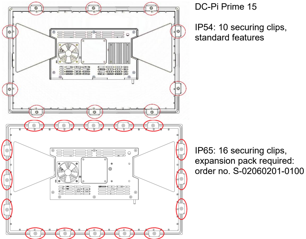
Fig. 34: Fully tightening the securing clips
