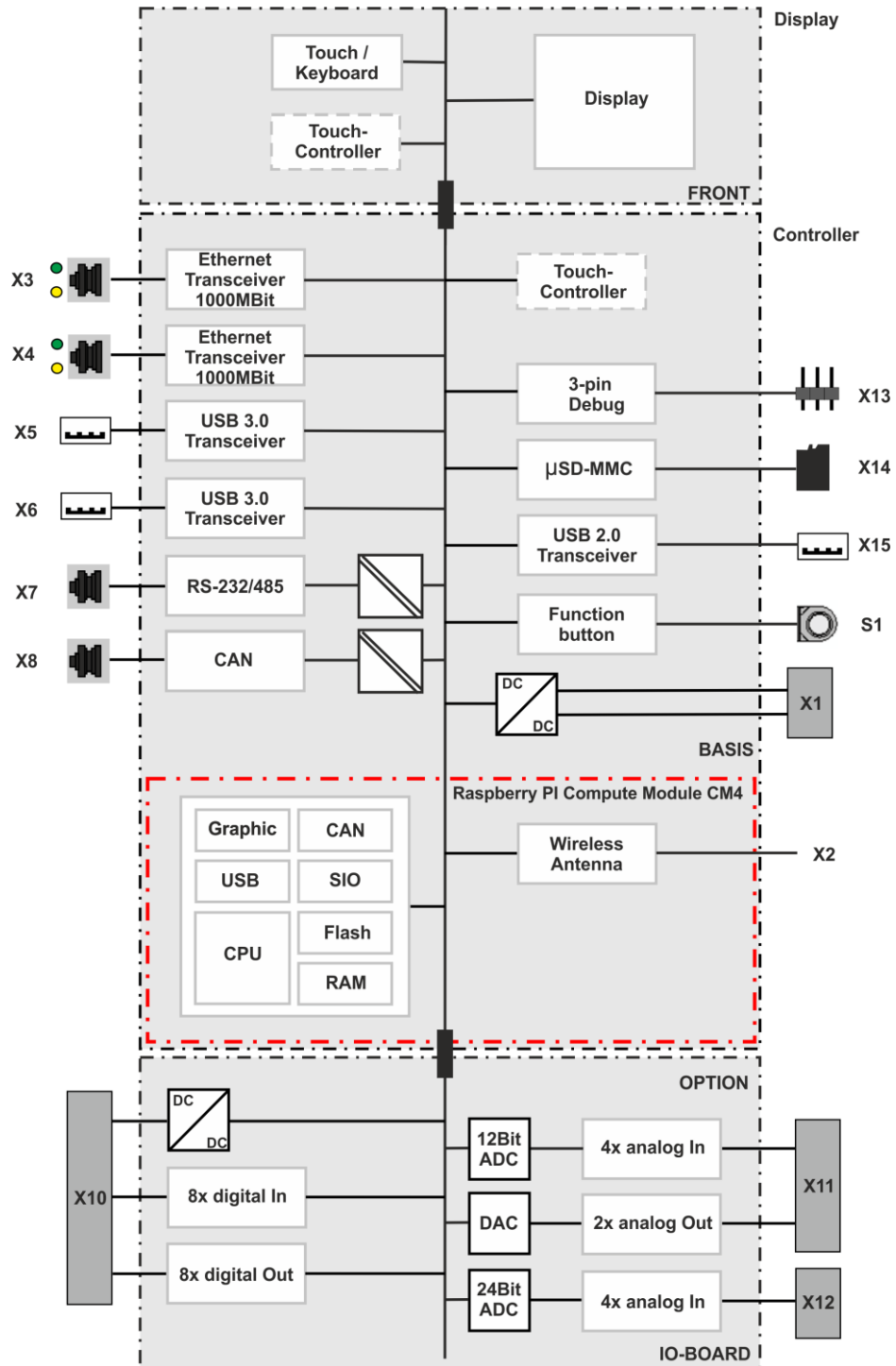
Fig. 13 : Block diagram DC-Pi Prime
