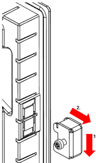
Fig. 35: Removing the securing clips
