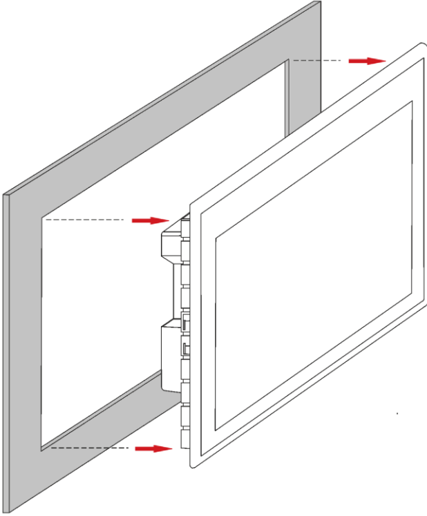
Fig. 36: Pushing the device out of the installation cut-out
