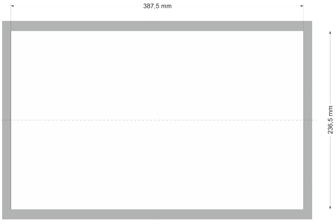
Fig. 8: DC-Pi Prime 15 mounting cut-out
