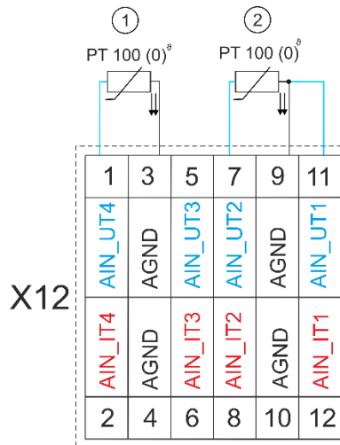
Fig. 23: Connection example: Temperature measurement
