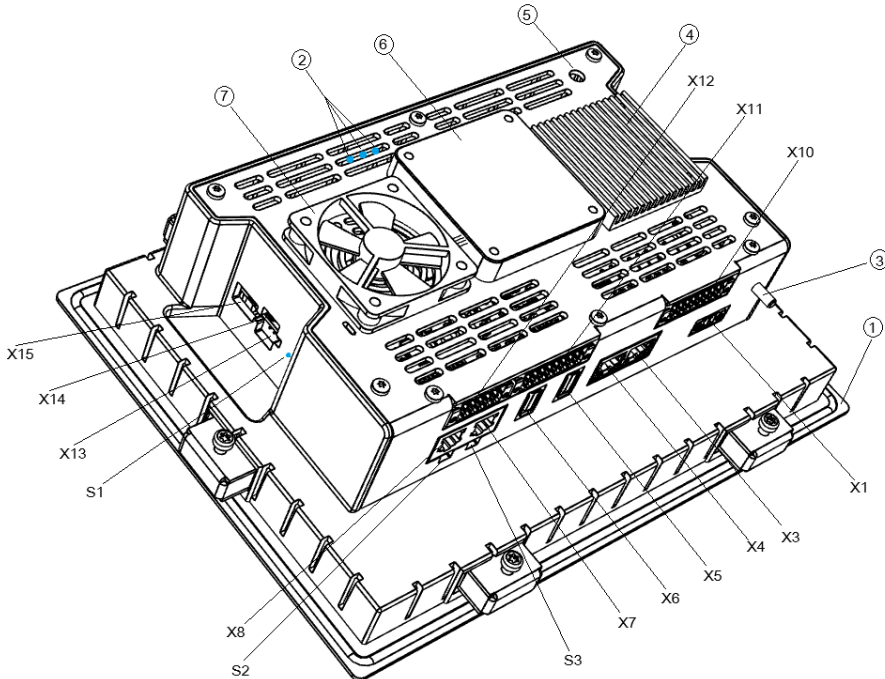
Fig. 2 : Overview of B-Primis DC-Pi Prime 10 S02-S04 (rear)
