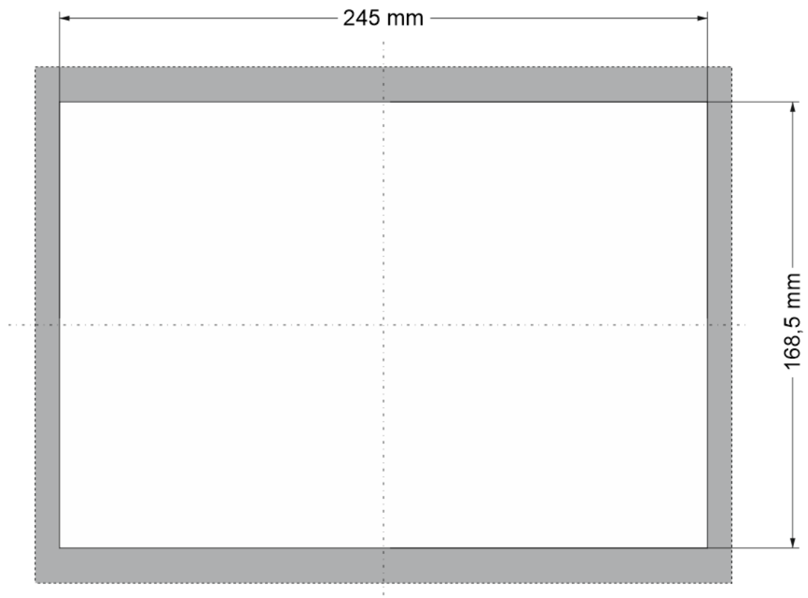
Fig. 6: DC-Pi Prime 10 mounting cut-out
