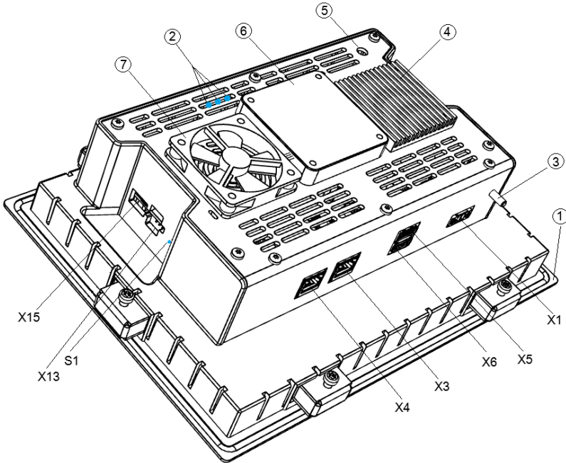
Fig. 1: Overview of B-Primis DC-Pi Prime 10 S01 (rear)
