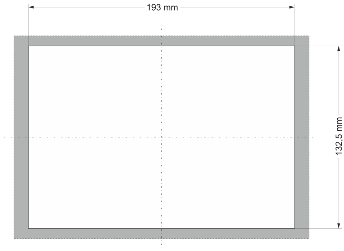
Fig. 4: DC-Pi Prime 7 mounting cut-out
