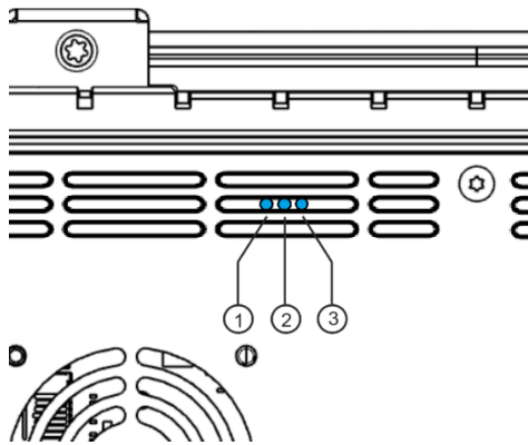
Fig. 29: Positions of the operating status LEDs
