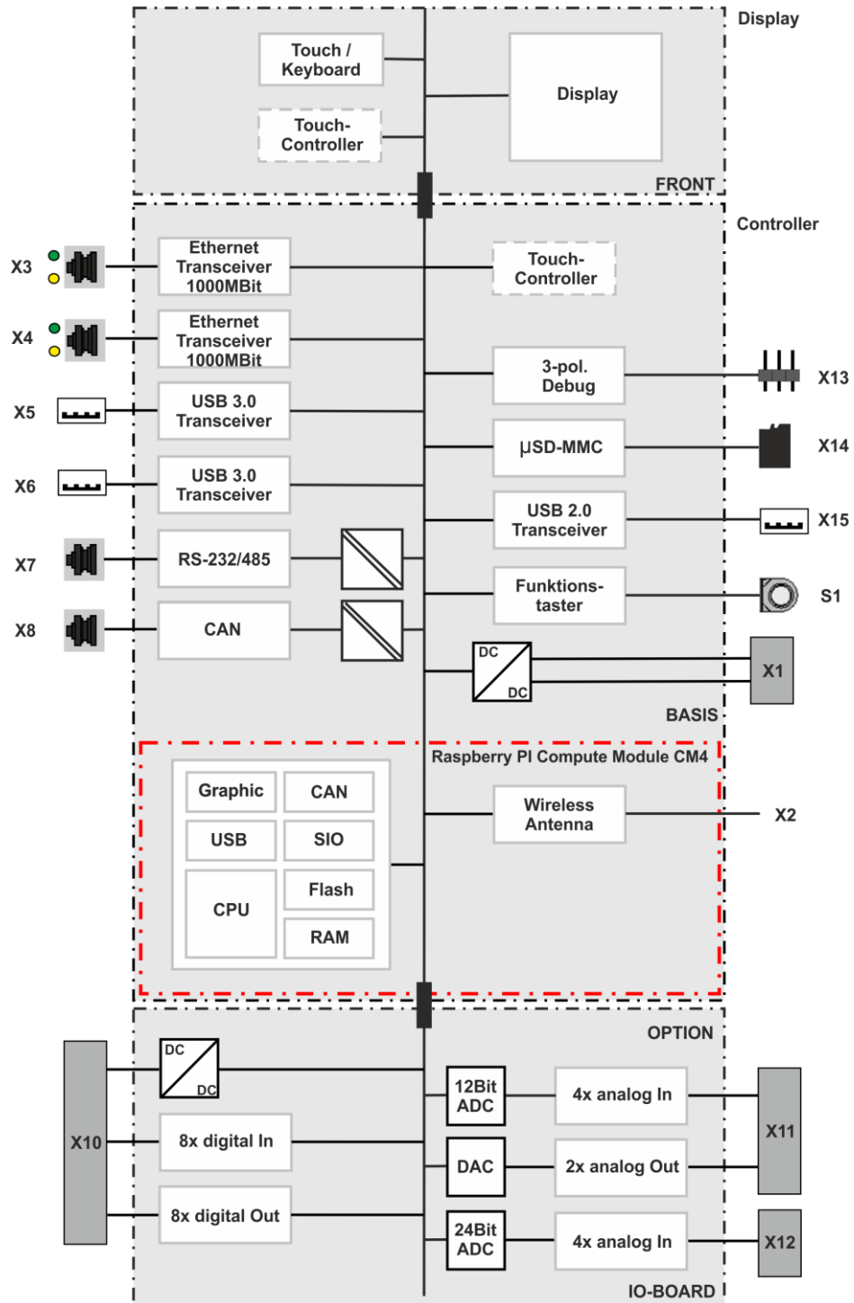
Fig. 13 : Block diagram DC-Pi Prime Open
