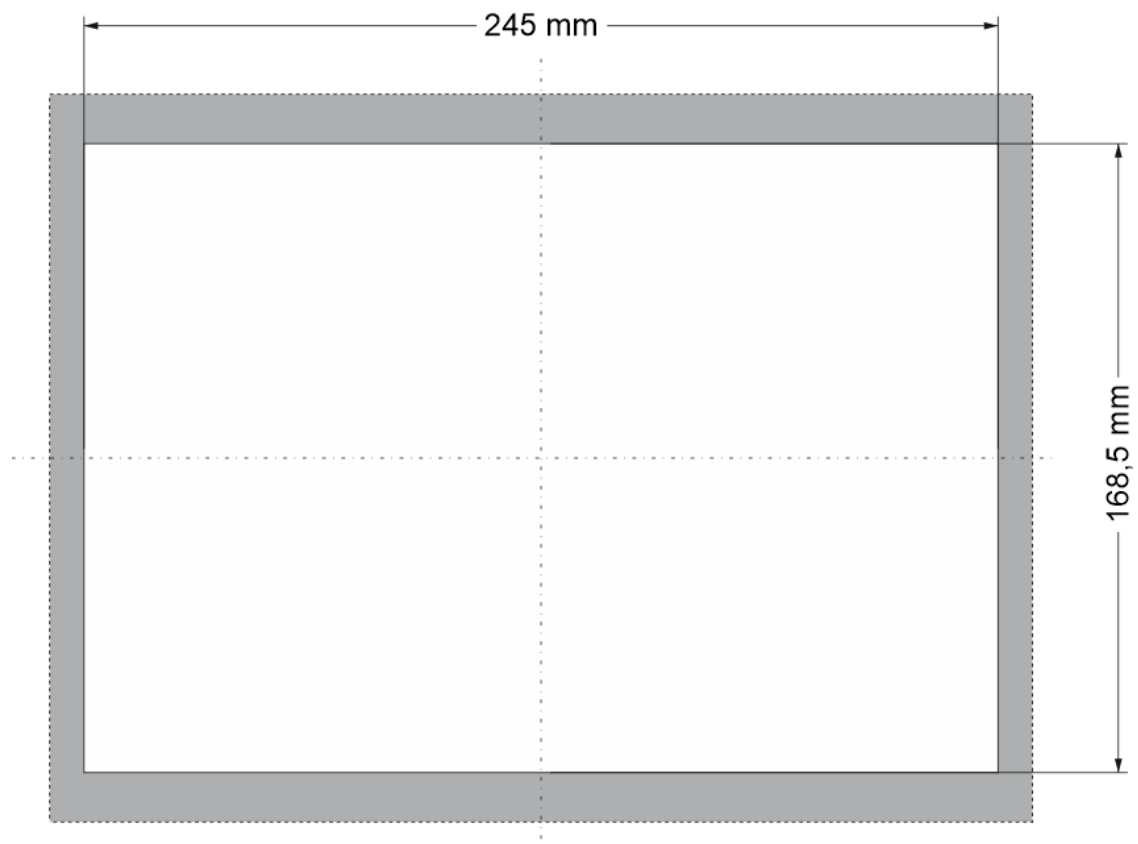
Fig. 6: DC-Pi Prime Open 10 mounting cut-out
