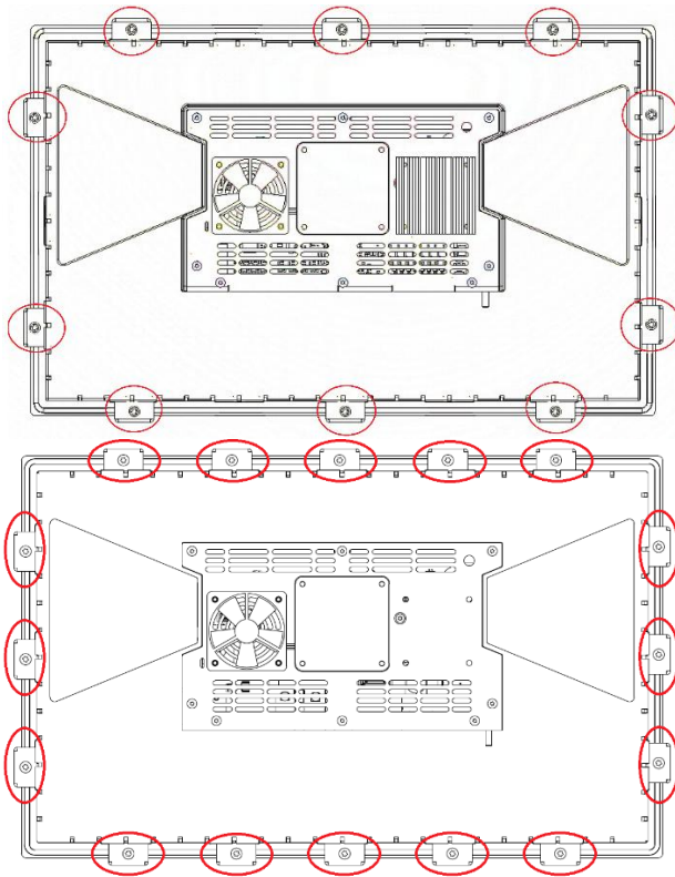
Fig. 31: Loosening the screws
