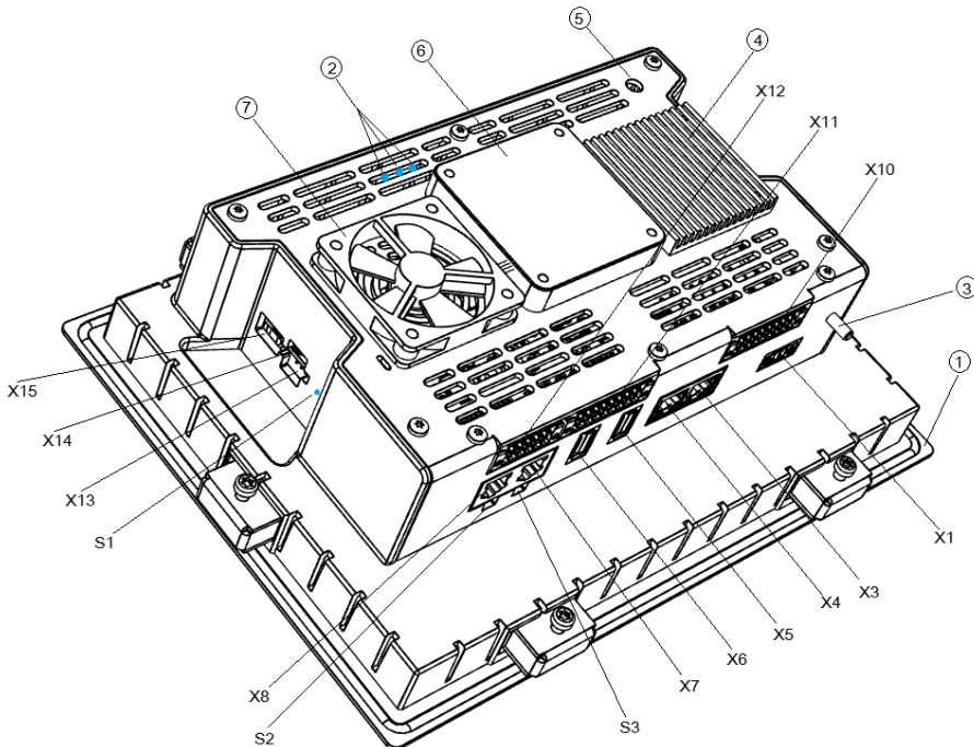
Fig. 2 : Overview of B-Primis DC-Pi Prime Open 10 S02-S04 (back)
