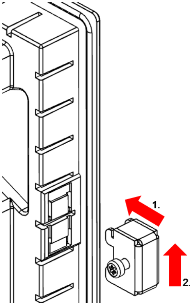
Fig. 10: Fitting the securing clip
