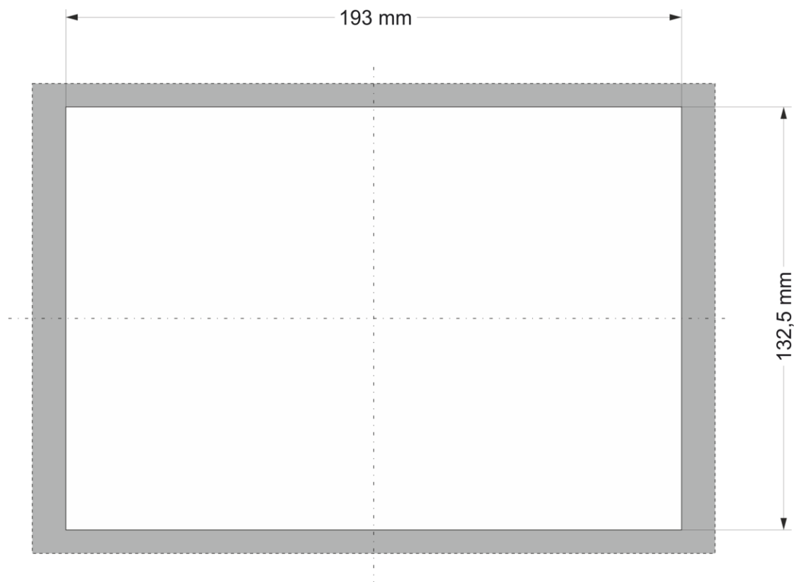
Fig. 4: DC-Pi Prime Open 7 mounting cut-out
