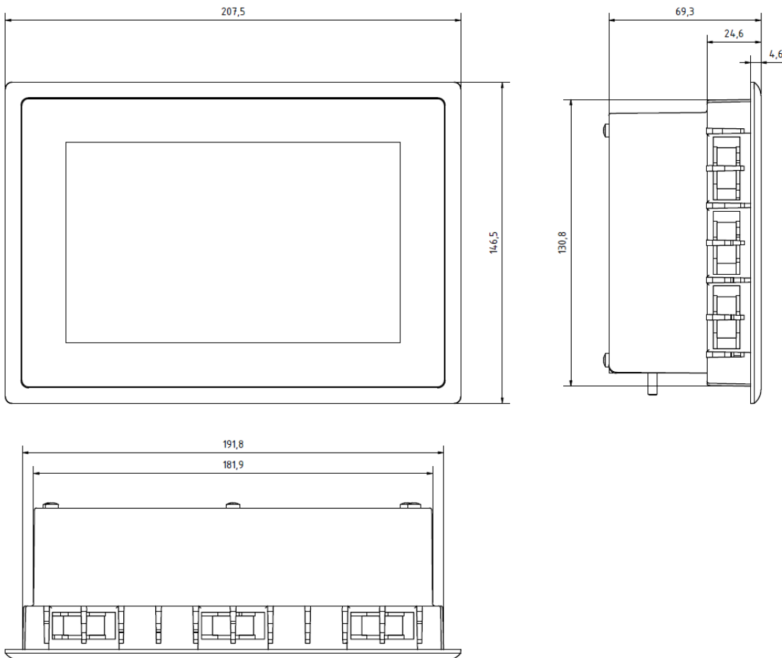
Fig. 3 : Dimensions DC-Pi Prime Open 7
