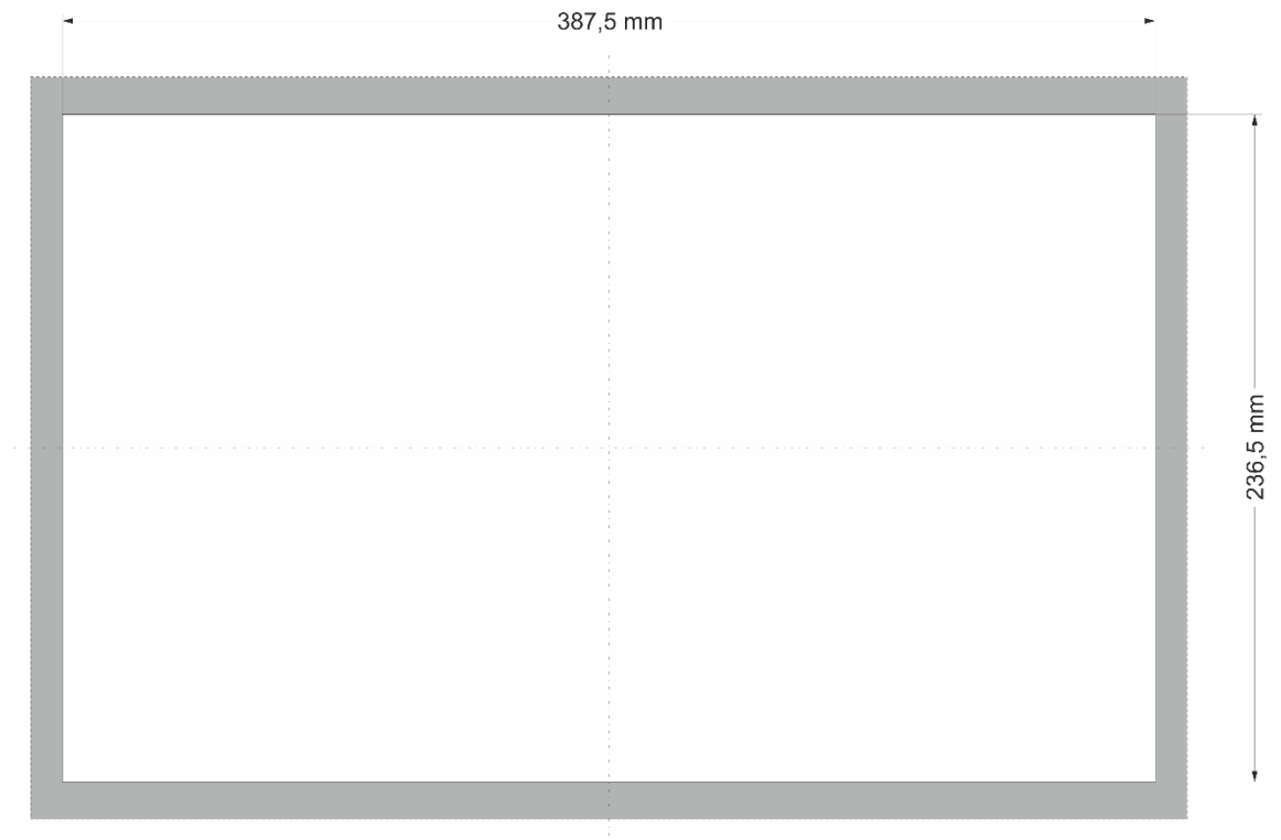
Fig. 8: DC-Pi Prime Open 15 mounting cut-out
