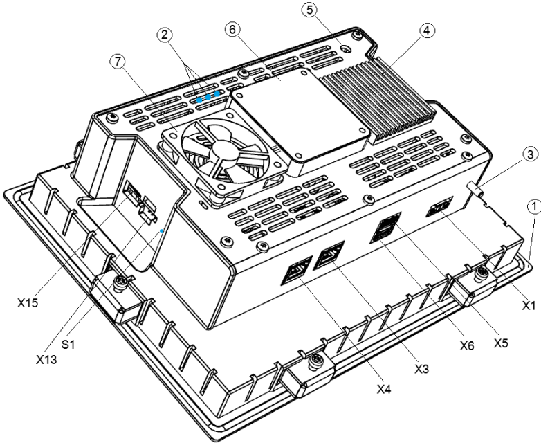
Fig. 1: Overview of B-Primis DC-Pi Prime Open 10 S01 (back)
