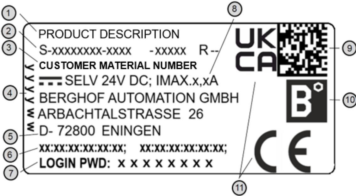
Fig. 34: Type plate
